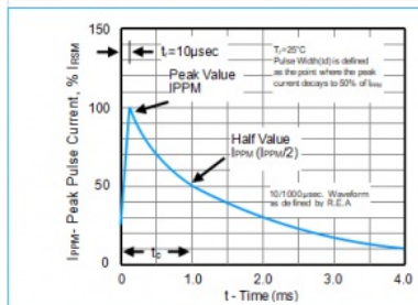
Figure 3 - Pulse Waveform
